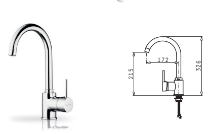
Single lever mixer tap with ceramic disc mechanism
