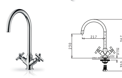
Dual lever mixer tap with ceramic disc mechanisms
